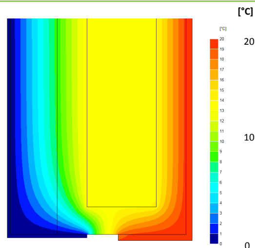
Temperature Distribution
